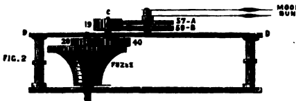
Section of the Astronomical Wheel-work of Ferguson's Solar and Lunar Watch.
